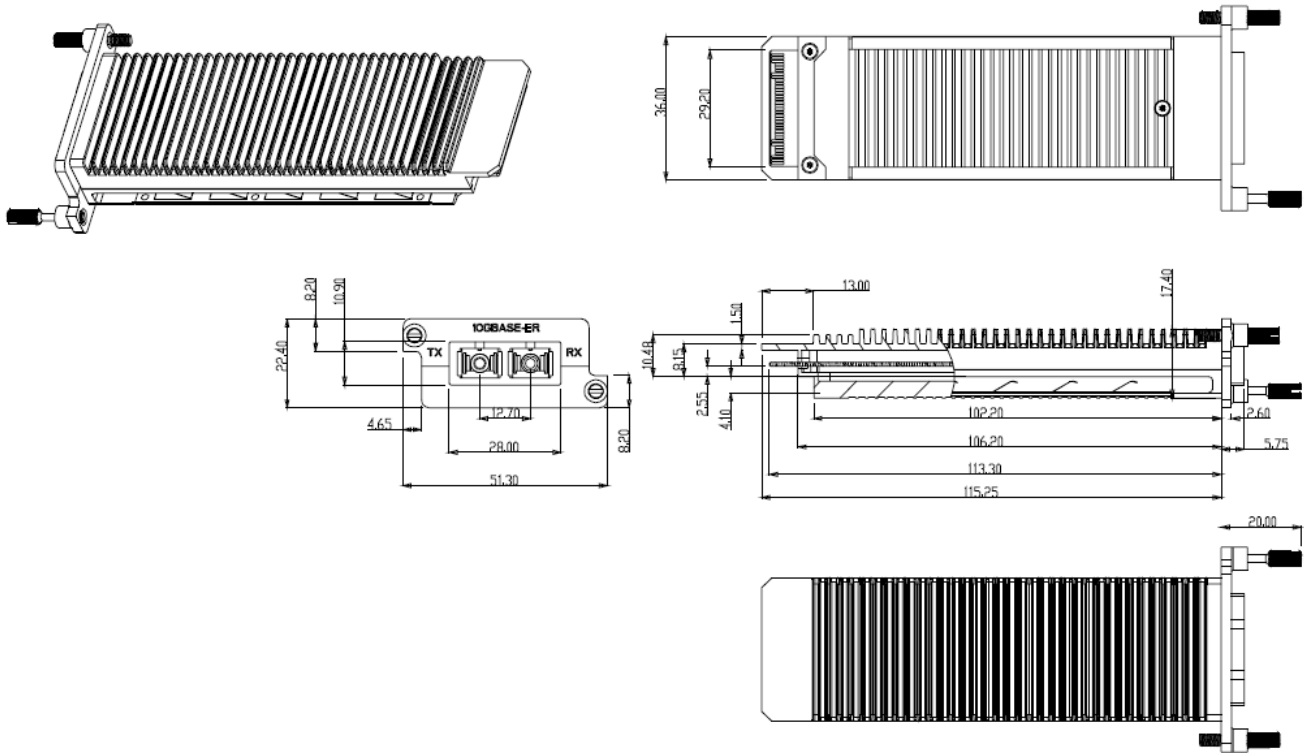
Figure2. Functional Diagram of Typical XENPAK Style Transceiver
