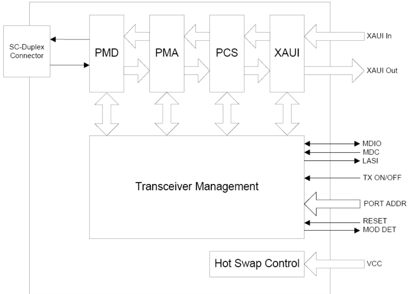
Figure1.Electrical Pin-out Details
