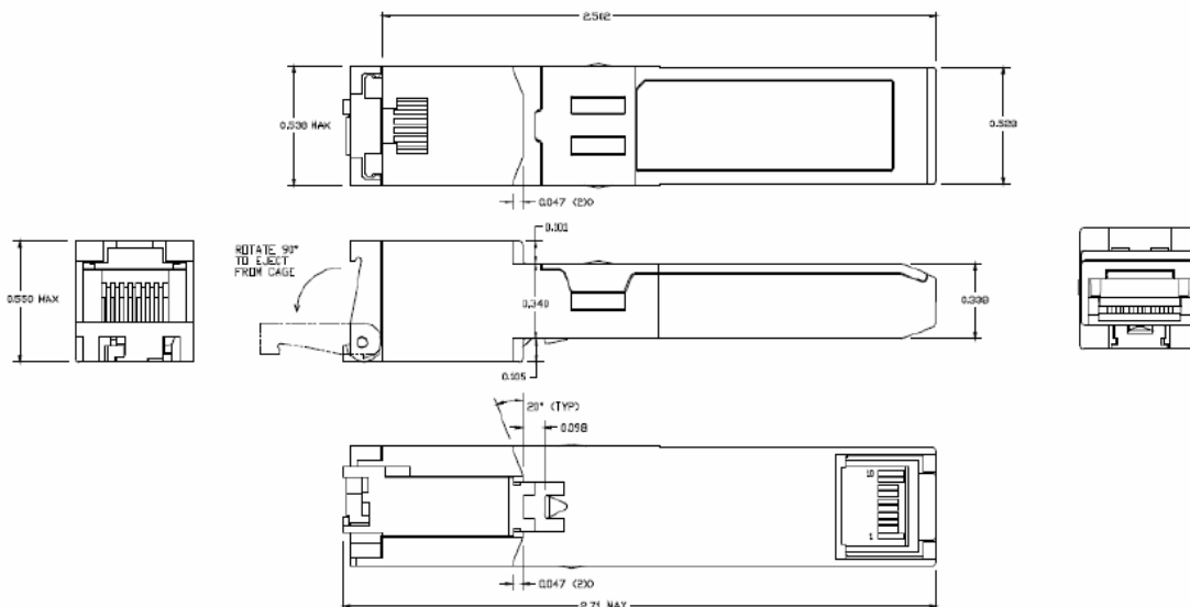
Figure 2. SPT-PE-T2 mechanical dimensions
